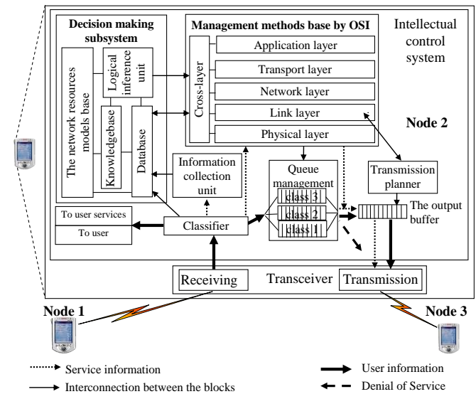
Fig. 3. Architecture of intellectual nodal control system
